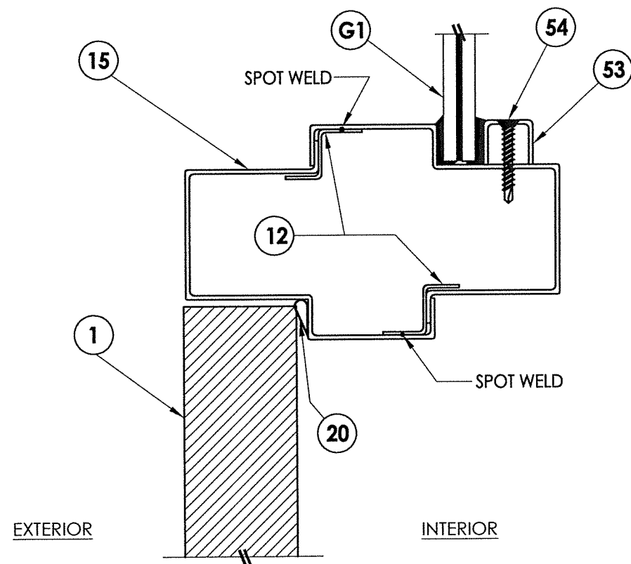
4 VERTICAL CROSS SECTION
