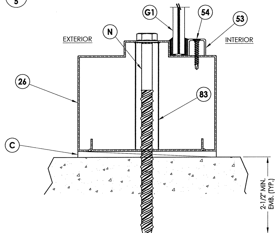
2 VERTICAL CROSS SECTION 5
