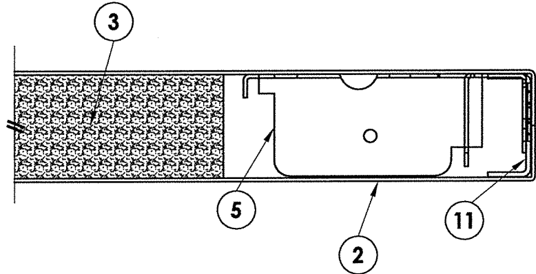
2 HORIZONTAL CROSS SECTION 2 Door panel
