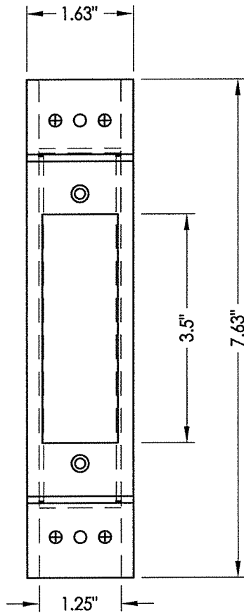
27 LATCH STRIKE REINFORCEMENT
