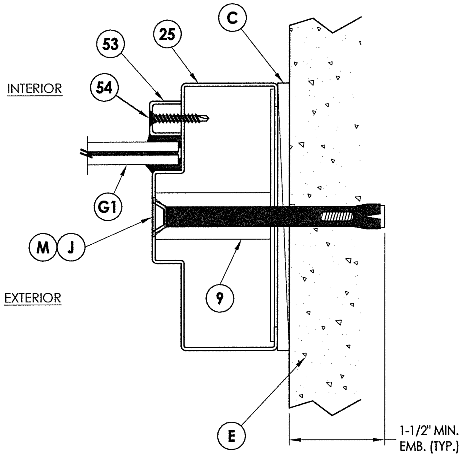
4 4 HORIZONTAL CROSS SECTION
