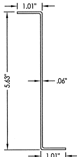
84 MULLION REINFORCEMENT
