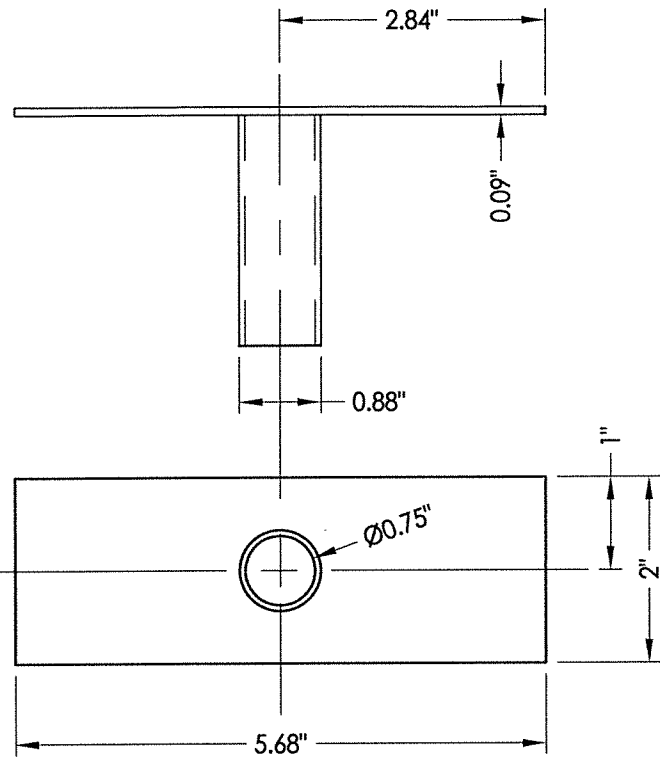
9 TUBE ANCHOR
